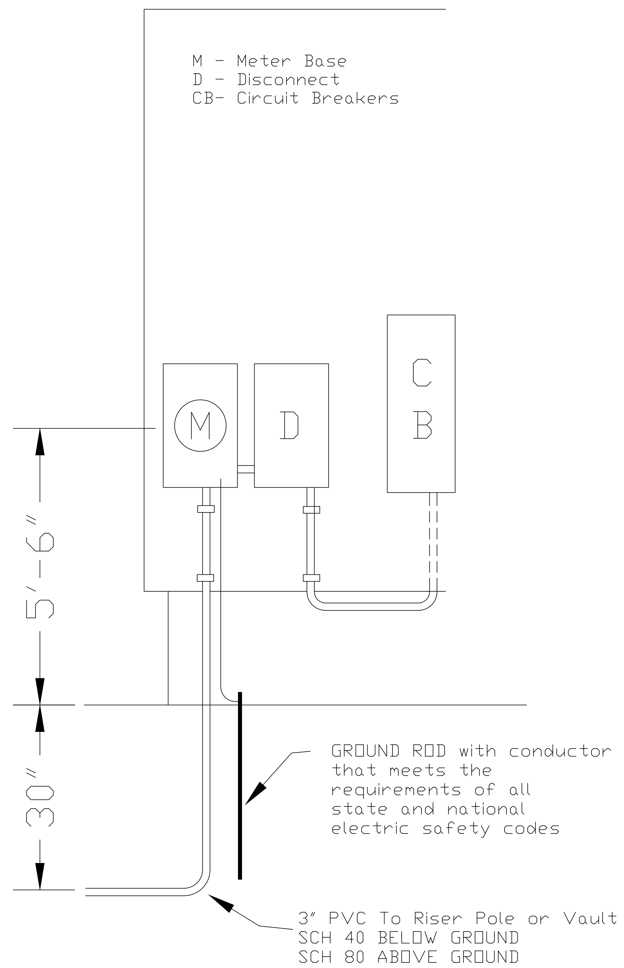
UNDERGROUND SERVICE TO MANUFACTURED/MODULAR HOME
